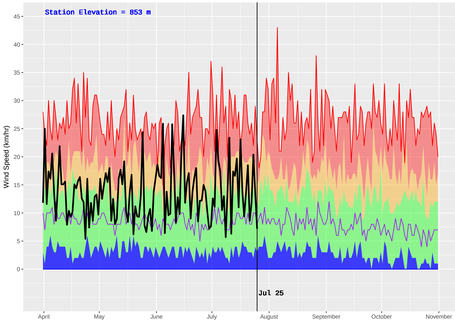
JOHNSON LAKE (419) : Historical (1986–2016) and Current (2017) Noon Wind Speed
